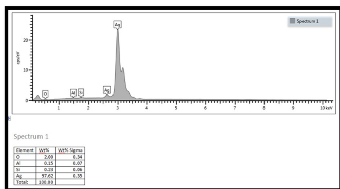
Figure 6. EDS Spectra Analysis of Sample Ag1
