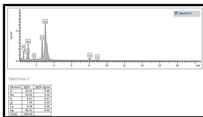
Figure 7. EDS Spectra Analysis of Sample Ag2
