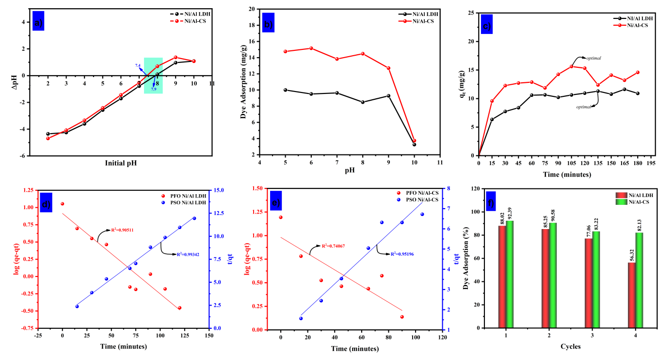
Figure 2. Determination of Adsorbent pHpzc (a), Effect of pH (b) and Contact Time (c) on MO Adsorption, Modeling of Adsorption Kinetics Using PFO and PSO Models for Ni/Al LDH (d) and Ni/Al-CS (e), and Study of Adsorbent Regeneration in the Adsorption Process (f)
