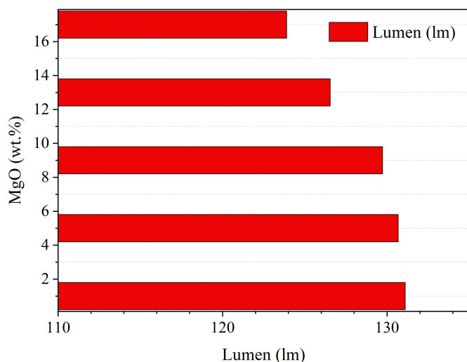
Figure 5. Luminescence Strength with Various MgO Proportions
