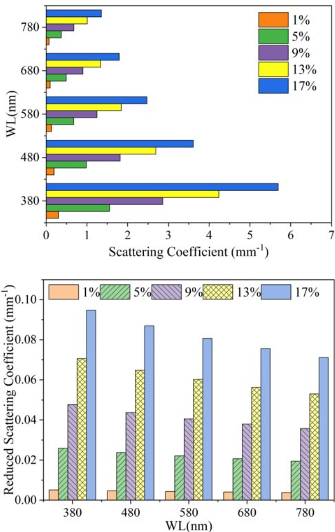
Figure 1. Scattering Coefficients with Various Wavelengths
