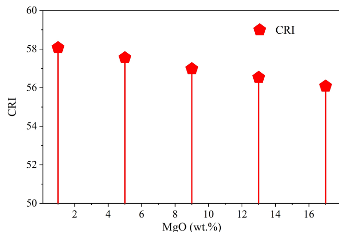
Figure 6. CRI Values with Various MgO Proportions
