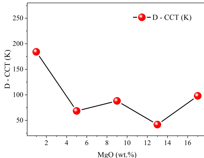
Figure 4. Color Difference Values with Different MgO Proportions
