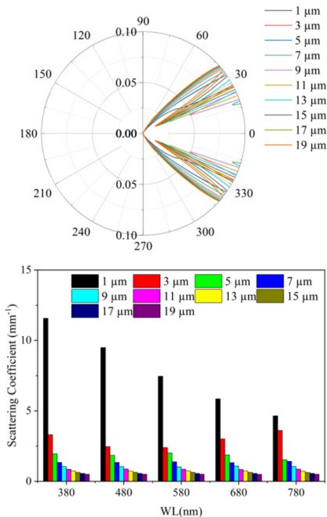
Figure 1. Relationship Between Scattering Coefficient and Wavelengths
